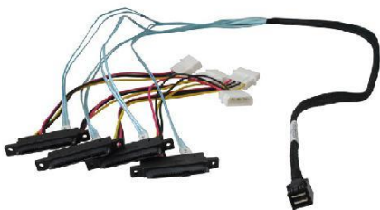
8643-4SAS-1M - 1 Meter Cable length, SFF-8643 to Controller and 4x SFF-8482 to 4x SAS Drives
